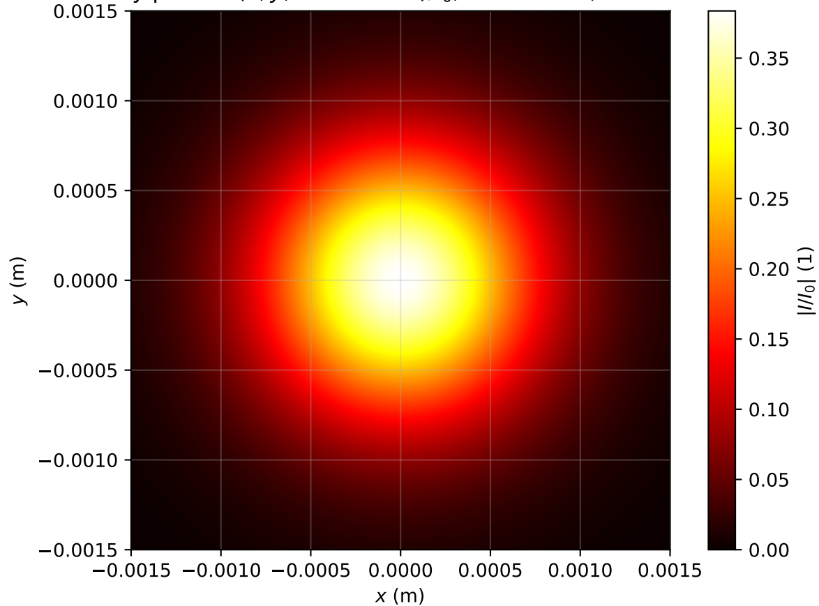
Intensity profile I(x, y, z = 3.582m)/I_0 , P_{in}=0.4P_{cr} , artificial time
